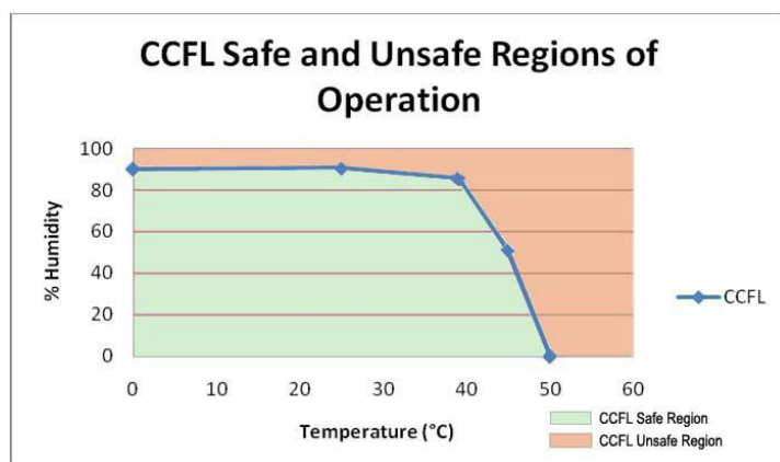
Figure 2: Relative Humidity Tolerance of CCFL Backlit HMI's. Note: Under the curve represents safe region and over the curve is the unsafe region of operation for CCFL backlit HMI's.
