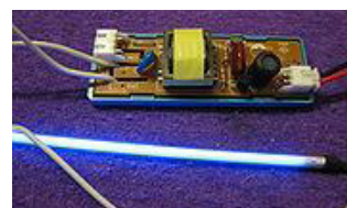
Figure 4: Example of a conventional CCFL inverter board and CCFL backlight bulb
